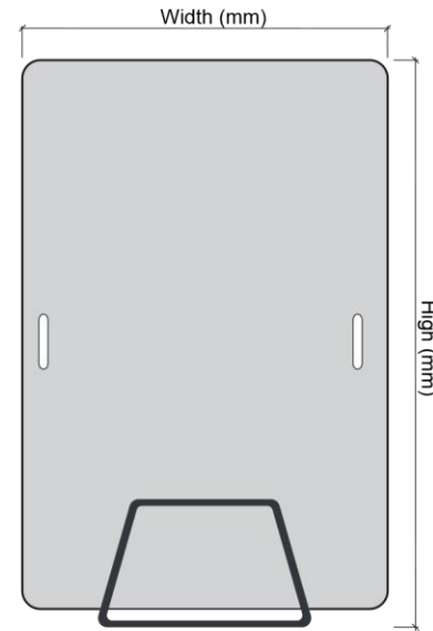
Front Acrylic (12mm thk) Width : 1000W (mm) High : 1500H (mm)
