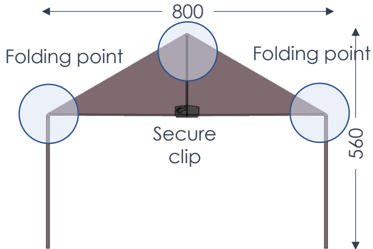
Top view – with canopy
