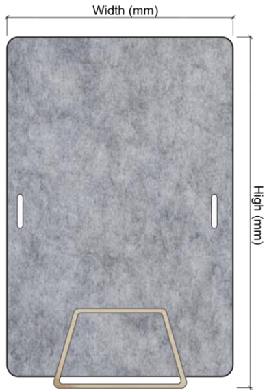
Front Ekous (12mm thk) Width : 1000W (mm) High : 1500H (mm)
