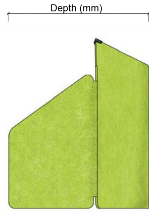
Side View (EKOUS 9mm Thk)
